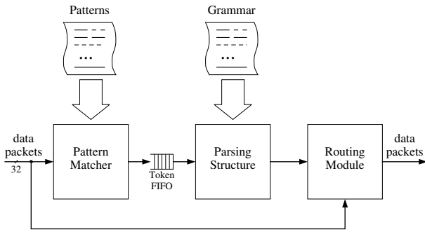
Figure 4. Content-based router architecture
