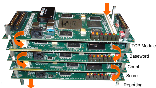
Figure 1 – A stack of five Field-programmable Port Extender (FPX) platforms built with a total of ten FPGAs (5 RADs and 5 NIDs) implement Automated Front End (AFE) processing Hardware.
