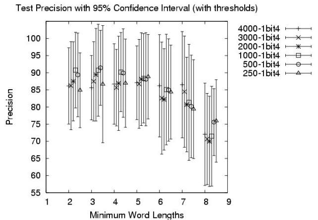
Figure 13 MI Algorithm Precision Results for 1 bit Count Resolution
