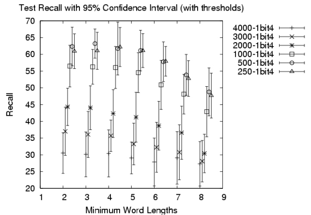
Figure 12 Heuristic Algorithm Recall Results for 1 bit Count Resolution
