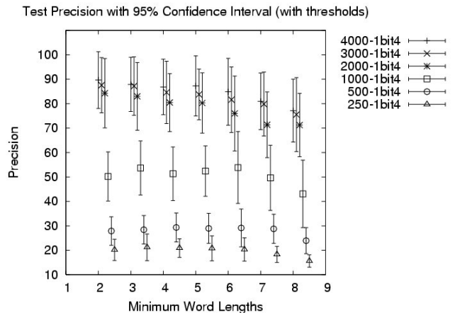
Figure 11 Heuristic Algorithm Precision Results for 1 bit Count Resolution
