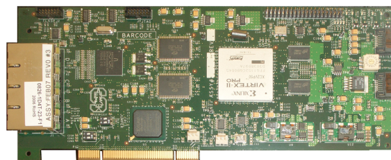
Figure 1. Photo of the NetFPGA 2.1
