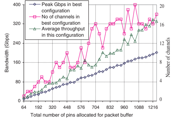
Fig. 8. Memory bandwidth as a function of pins when the buffer is designed to maximize worst case performance.
