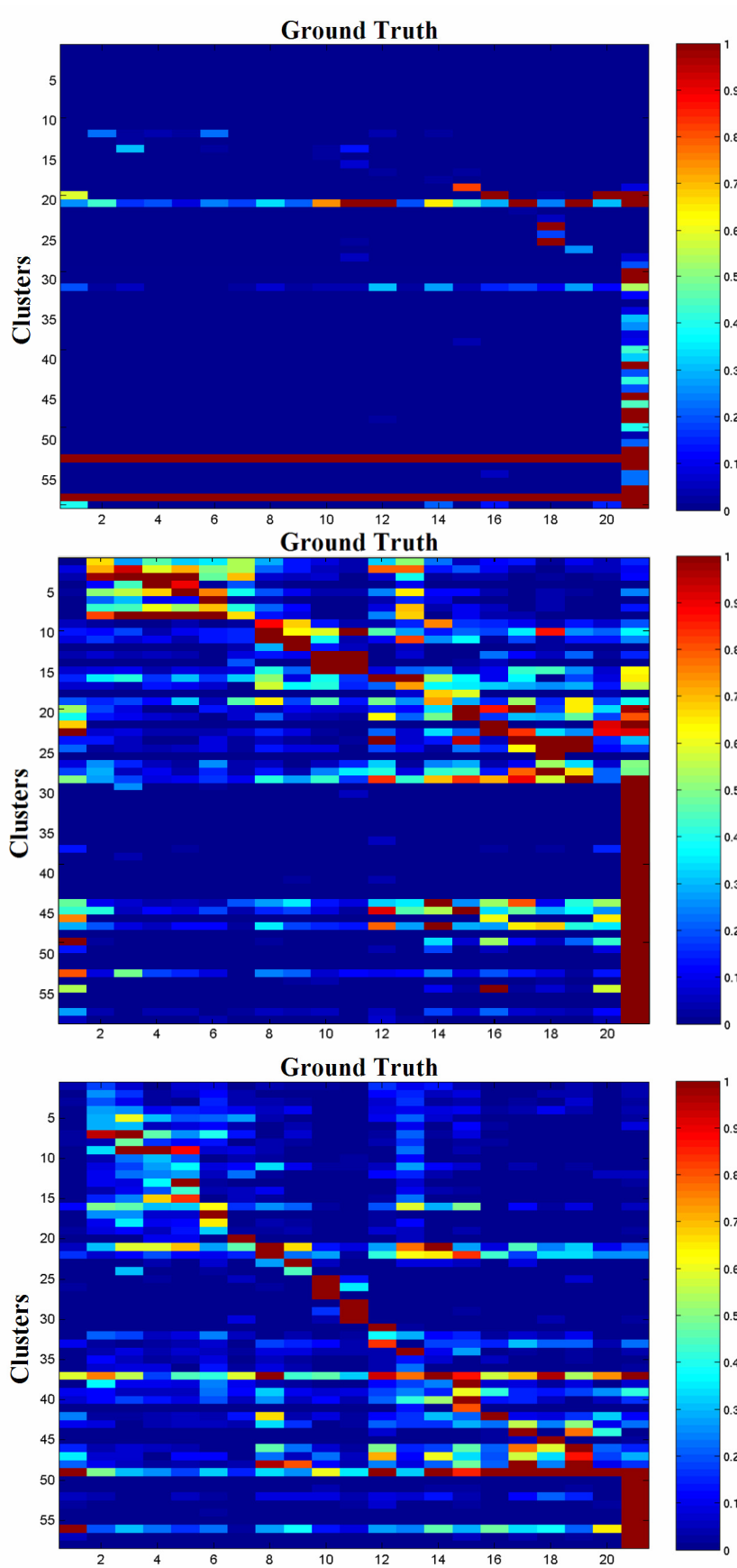
Figure 3 – Confusion matrices for k-means (top), bisectonal k-means (middle), and hierarchical partitioning (bottom), on the dataset of 23,845 newsgroup postings described in the text.
