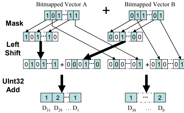
Figure 4: 32-dimension vector sum using Integer operations. The vector sum is accomplished using 6 instructions instead of 32x2=64 instructions.
