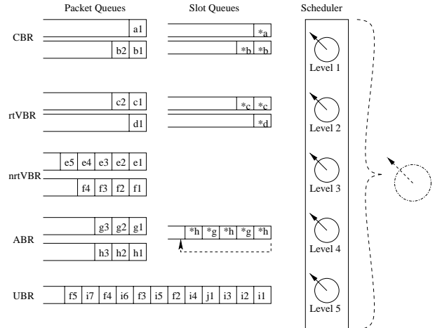
Figure 2: MPFQ Base Station Scheduler
