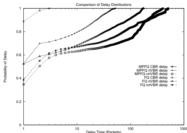
Figure 3: Cumulative Distribution of Delay
