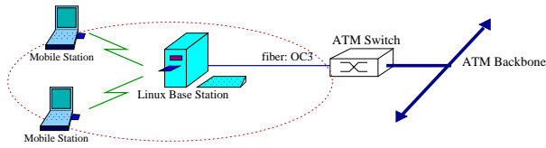
Figure 1: Scheduler Testbed
