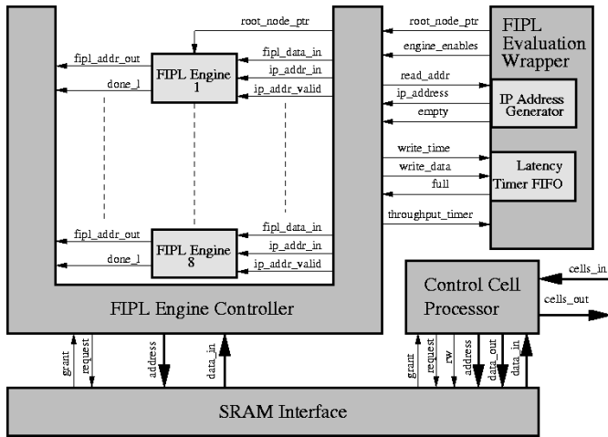
Fig. 13. Block diagram of FIPL evaluation environment.
