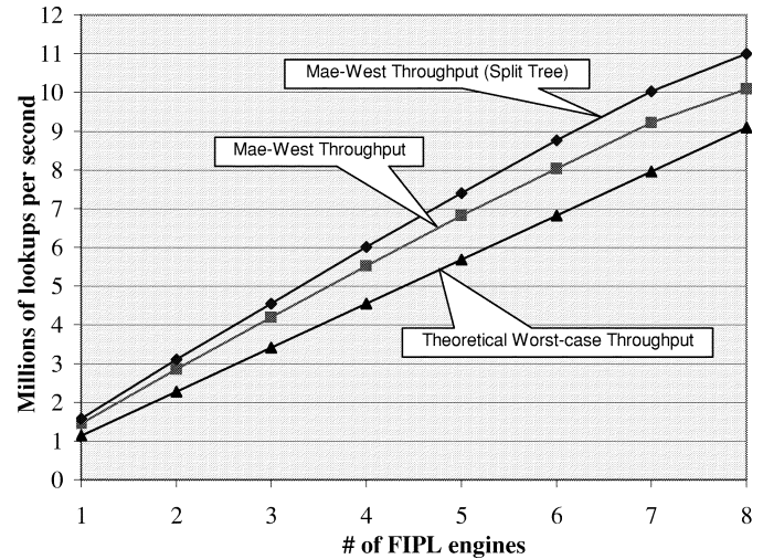
Fig. 14. FIPL performance: measurements used a snapshot of the Mae-West database from March 15, 2002, consisting of 27 609 routes. Input IPv4 destination addresses were created by randomly selecting 16 384 prefixes from the Mae-West database.
