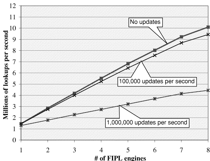
Fig. 15. FIPL performance under update load: measurements used a snapshot of the Mae–West database from March 15, 2002, consisting of 27 609 routes. Input IPv4 destination addresses were created by randomly selecting 16 384 prefixes from the Mae–West database. Updates consisted of alternating addition and deletion of a 24-bit prefix.
