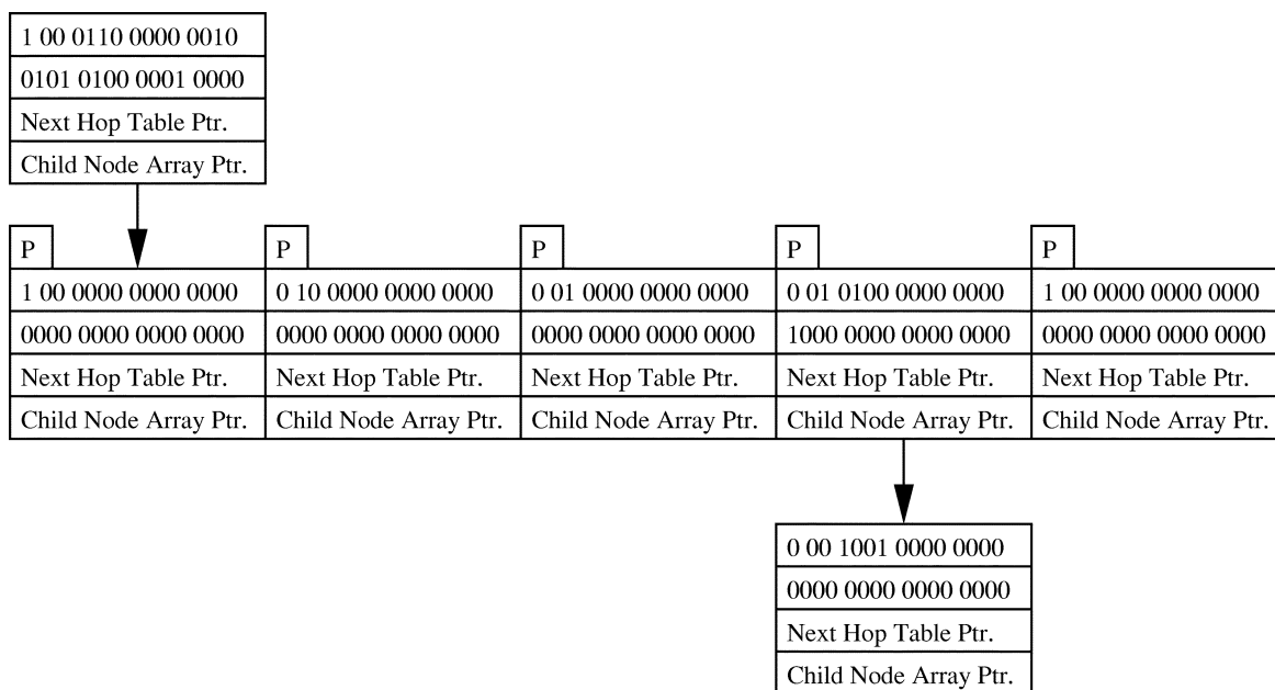
Fig. 5. IP lookup table represented as a Tree Bitmap. Child nodes are stored contiguously so that a single pointer and an index may be used to locate any child node in the data structure.
