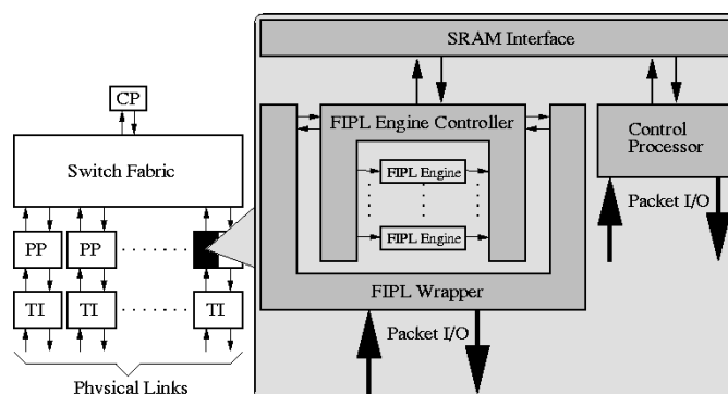
Fig. 7. Block diagram of router with multiengine FIPL configuration; detail of FIPL system components in the port processor (PP).
