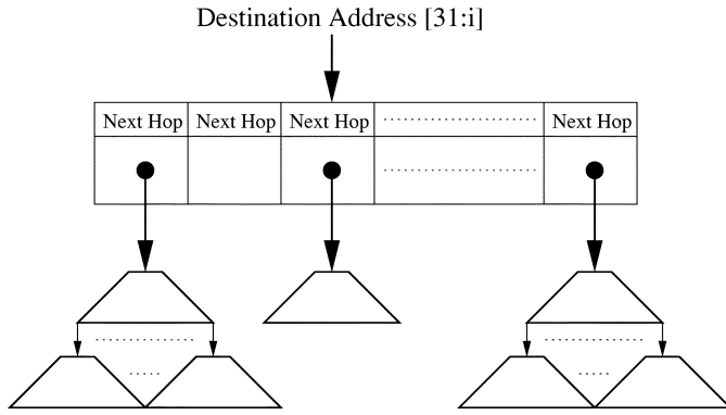
Fig. 17. Root node extension using an on-chip array and multiple sub-tries.
