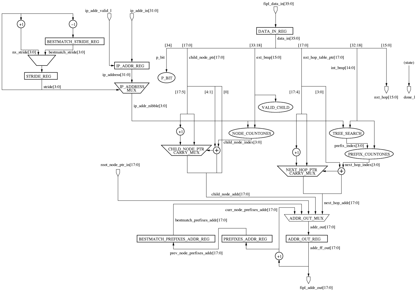
Fig. 8. FIPL engine dataflow; multicycle path from input data flops to output address flops can be scaled according to target device speed; all multiplexor select lines and flip-flop enables implicitly driven by finite-state machine (FSM) outputs.
