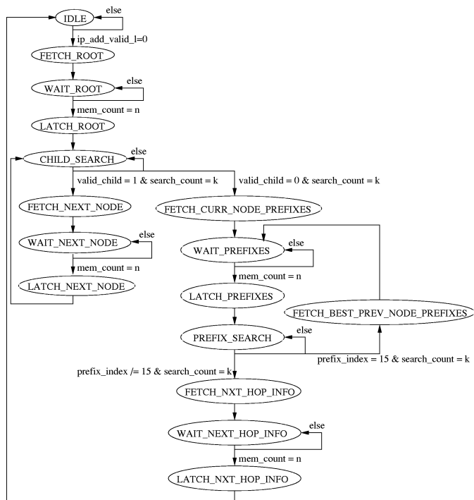
Fig. 9. FIPL engine state transition diagram.
