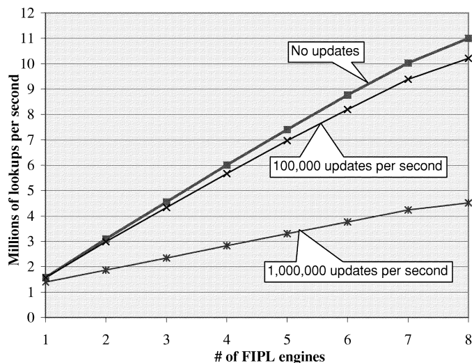
Fig. 16. FIPL split-trie performance under update load: measurements used a snapshot of the Mae–West database from March 15, 2002, consisting of 27 609 routes. Input IPv4 destination addresses were created by randomly selecting 16 384 prefixes from the Mae–West database. Updates consisted of alternating addition and deletion of a 24-bit prefix.
