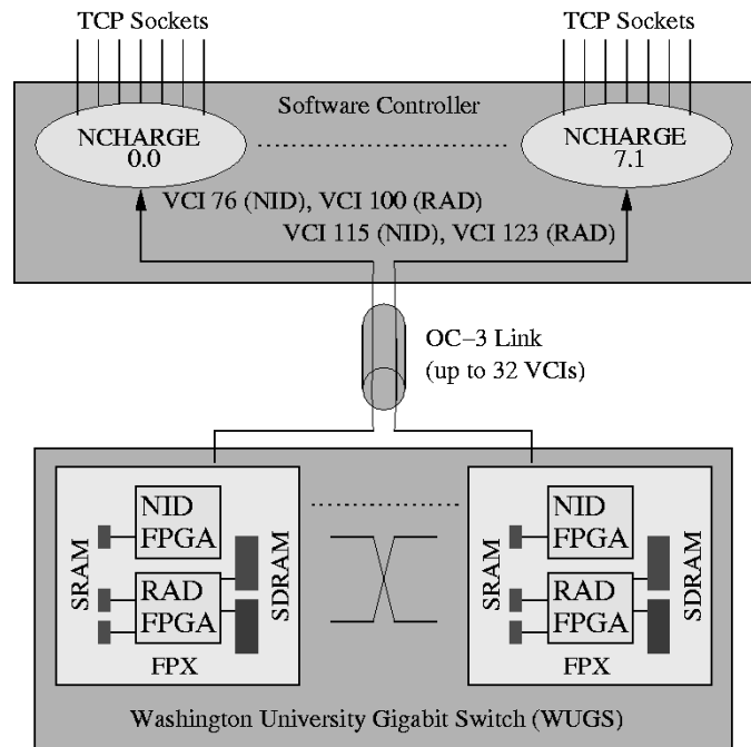
Fig. 10. Control of the FPX via NCHARGE software. Each FPX is controlled by an instance of NCHARGE which provides an API for FPX control via remote software process.
